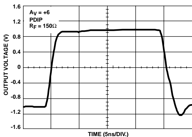
FIGURE 45. LARGE SIGNAL PULSE RESPONSE
