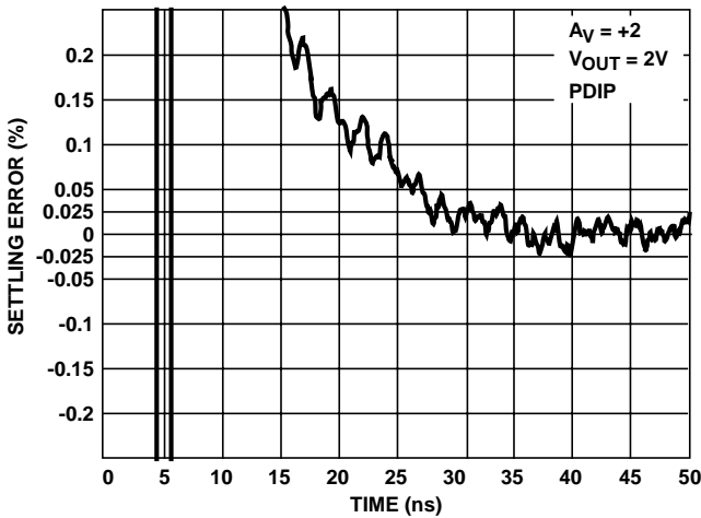
FIGURE 54. SETTLING RESPONSE
