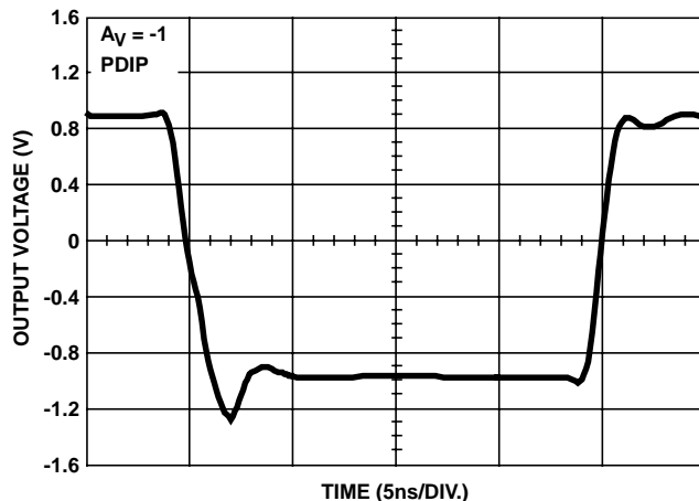
FIGURE 41. LARGE SIGNAL PULSE RESPONSE
