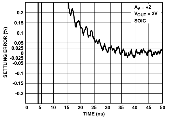
FIGURE 19. SETTLING RESPONSE
