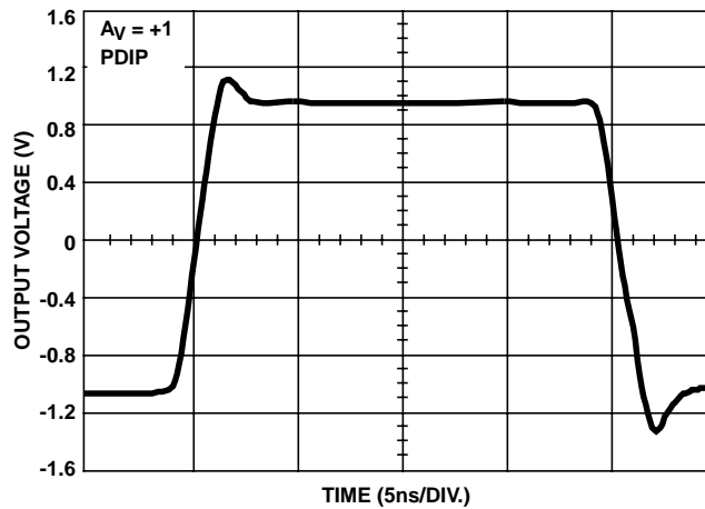
FIGURE 43. LARGE SIGNAL PULSE RESPONSE
