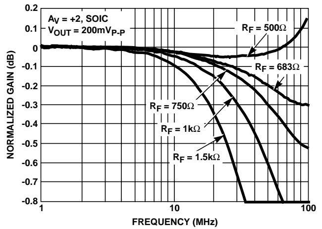
FIGURE 17. GAIN FLATNESS vs FEEDBACK RESISTOR
